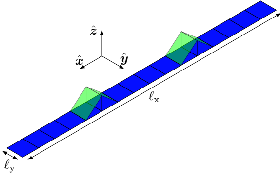
Fig. 10. A thin strip dipole with dimensions \ell_x , \ell_y divided into N_x = 16 rectangular mesh elements. Two piecewise linear divergence conforming basis functions are depicted.
