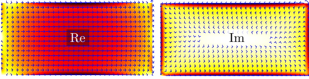
Fig. 23. Resulting current density for the G/Q problem in Fig. 22. Real and imaginary parts to the left and right, respectively. The real part is dominated by an \hat{x} -directed current radiating as an \hat{x} -directed electric dipole. The imaginary part is a loop type current that radiates as a \hat{z} -directed magnetic dipole (see also Fig. 24).
