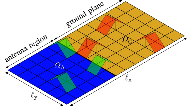
Fig. 8. Illustration of discretization for a region \Omega using rectangular mesh elements. The region is divided into the antenna region ( \Omega_A ) and ground plane region, \Omega_G . The amplitudes of six basis functions (18), three (green) in \Omega_A and three (red) in \Omega_G , are depicted. We let overlapping basis functions belong to the antenna part.
