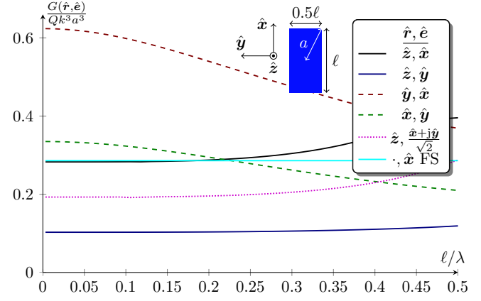
Fig. 18. Gain Q-factor quotient, G/Q , from the optimization problem (39) for a rectangular plate with side lengths \ell and \ell/2 , wavelength \lambda \geq 2\ell , \hat{\mathbf{r}} = \{\hat{\mathbf{x}}, \hat{\mathbf{y}}, \hat{\mathbf{z}}\} and \hat{\mathbf{e}} = \{\hat{\mathbf{x}}, \hat{\mathbf{y}}, (\hat{\mathbf{x}} + j\hat{\mathbf{y}})/\sqrt{2}\} . The G/Q is normalized with k^3 a^3 , where a = \ell\sqrt{5}/4 is the radius of the smallest circumscribing sphere.
