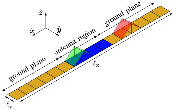
Fig. 13. A thin strip dipole with dimensions \ell_x , \ell_y divided into N_x = 16 rectangular mesh elements. The region is decomposed into the antenna region \Omega_A in the center with 4 elements and the surrounding PEC ground plane region \Omega_G at the edges with totally 12 elements. The corresponding basis functions are divided into 5 basis functions in the antenna region \Omega_A and 10 basis functions in \Omega_G . Two basis functions are depicted, one in \Omega_A (green) and one in \Omega_G (red).
