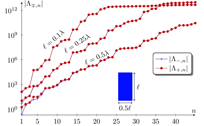
Fig. 27. The smallest 45 eigenvalues |\Lambda_{\mp,n}| of (77) for the planar rectangle with \ell = \ell_x = 2\ell_y and \ell = \{0.1, 0.25, 0.5\}\lambda . The rectangle is discretized with N_x = 2N_y = 64 equidistant elements (see Fig. 26).
