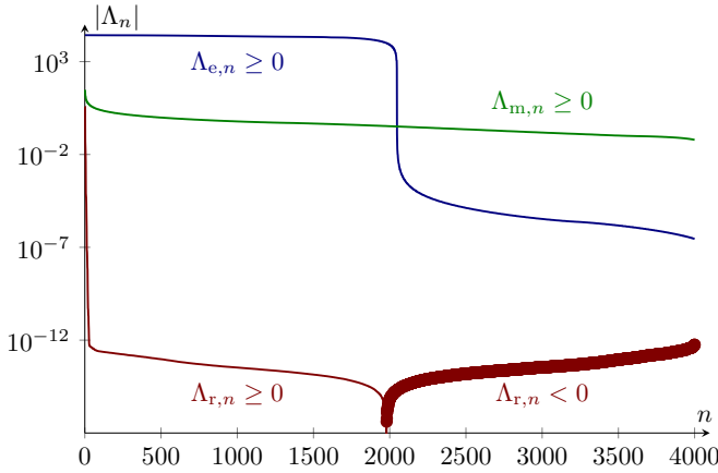
Fig. 28. Eigenvalues \Lambda_n of \mathbf{X}_e , \mathbf{X}_m , \mathbf{R} for a planar rectangle with side lengths \ell_x = 2\ell_y = 0.1\lambda divided into 64 \times 32 elements (4000 basis functions).
