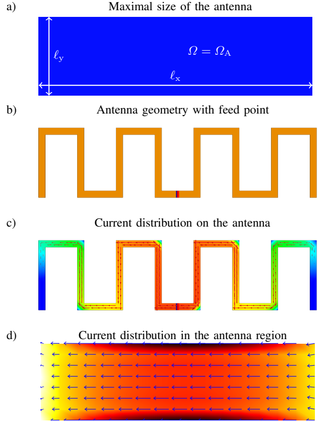
Fig. 3. Antenna and current optimization. In antenna optimization, we design antennas with optimal performance. In current optimization, we synthesize current densities with optimal performance. a) maximal antenna region. b) possible antenna design. c) current density on the antenna structure. d) possible current density in the antenna region.
