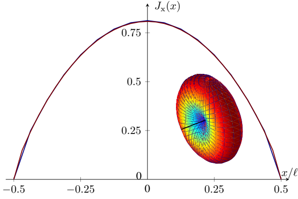
Fig. 11. The optimized current distribution on the strip dipole with length \ell and width \ell/50 discretized with N_x = \{16, 32\} rectangles in the blue and red curves for the half wavelength case \ell/\lambda = 0.48 (wavenumber k\ell \approx 3 ). The radiation pattern, with D(\hat{z}, \hat{x}) \approx 1.64 , is also depicted.
