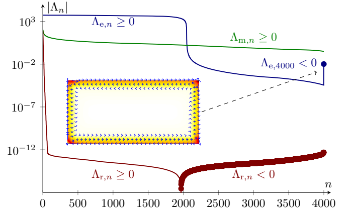
Fig. 29. Eigenvalues \Lambda_n of \mathbf{X}_e , \mathbf{X}_m , \mathbf{R} for a planar rectangle with side lengths \ell and \ell/2 divided into 64 \times 32 elements (4000 basis functions) for the wavelength \lambda = 2\ell . The negative eigenvalues are marked by circles, i.e. , \Lambda_n < 0 . The eigenmode (current) to the negative eigenvalue \Lambda_{e,4000} is also depicted, cf. , with the loop current in [35].
