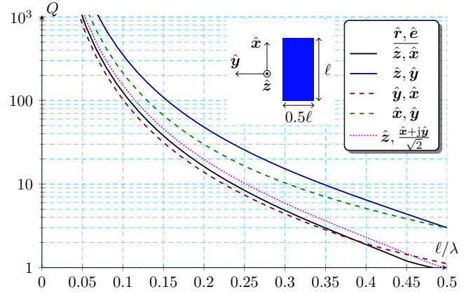
Fig. 19. Resulting Q from the optimization problem (39) for a rectangular plate with side lengths \ell and \ell/2 , electrical size \ell/\lambda \leq 0.5 , directions \hat{\mathbf{r}} = \{\hat{\mathbf{x}}, \hat{\mathbf{y}}, \hat{\mathbf{z}}\} and polarizations \hat{\mathbf{e}} = \{\hat{\mathbf{x}}, \hat{\mathbf{y}}, (\hat{\mathbf{x}} + j\hat{\mathbf{y}})/\sqrt{2}\} (see Fig. 18).
