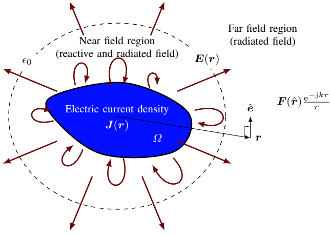
Fig. 2. Reactive and radiated fields from a current density \mathbf{J}(\mathbf{r}) in the region \Omega [37]. The reactive fields are concentrated in the near-field region around \Omega and vanish far from the source region \Omega , where \mathbf{E}(\mathbf{r}) \approx \mathbf{F}(\hat{\mathbf{r}})e^{-jkr}/r .
