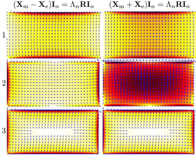
Fig. 26. Eigenmodes associated to the three smallest magnitudes of generalized eigenvalues of (\mathbf{X}_m \mp \mathbf{X}_e)\mathbf{I}_n = \Lambda_n \mathbf{R} \mathbf{I}_n for a planar rectangle with side lengths \ell and \ell/2 and wavelength \lambda = 10\ell . The rectangle is discretized with N_x = 2N_y = 32 equidistant elements.
