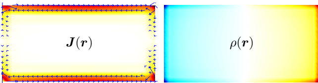
Fig. 21. Resulting current density and charge density for the rectangular plate in Fig. (20). The current density is \hat{x} -directed and strongest at the edges. The charge density distribution is close to the charge density on a PEC plate in a static electric field [35].
