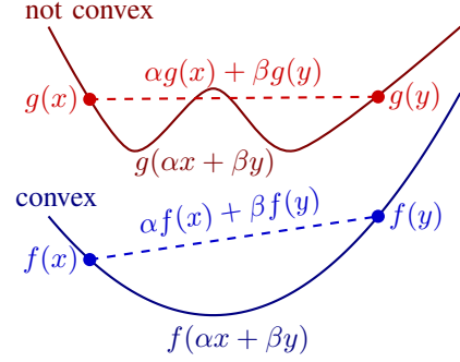
Fig. 9. Convex and non-convex functions. Convex functions satisfy f(\alpha\mathbf{x} + \beta\mathbf{y}) \leq \alpha f(\mathbf{x}) + \beta f(\mathbf{y}) for \alpha + \beta = 1 and \alpha, \beta \geq 0 , i.e., the curve is below the straight line between two points (see [6] for details). Note that the non-convex function g is convex if the domain is restricted to the left or right of the local maximum in the middle.
