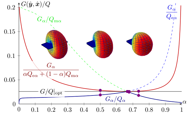
Fig. 22. G_\alpha/Q_\alpha from (56) for the plate in Fig. 19, \ell_x = 2\ell_y = 0.1\lambda , \hat{r} = \hat{y} and \hat{e} = \hat{x} . The resulting current distribution is depicted in Fig. 23. The radiation pattern is depicted for three values of \alpha , see also Fig. 24. The maximal value is G/Q|_{\text{opt}} \approx 0.0259 giving Q \approx 102 and D \approx 2.66 .
