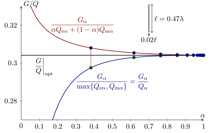
Fig. 15. Gain Q-factor quotient, G/Q , from the dual optimization problem (54) with the inequalities (56) for a strip dipole with size \ell \times \ell/50 , \ell/\lambda = 0.47 , \hat{\mathbf{r}} = \hat{\mathbf{z}} and \hat{\mathbf{e}} = \hat{\mathbf{x}} .
