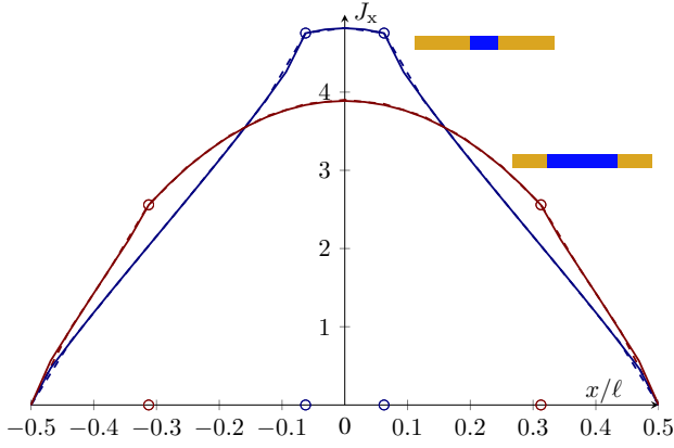
Fig. 14. The optimized current density distribution on the strip dipole with length \ell and width \ell/50 discretized with N_x = \{16, 32\} rectangles in the blue and red curves for the case \ell/\lambda = 0.1 (wavenumber k\ell \approx 0.63 ). The antenna region consists of the 2 (blue curve) and 10 (red curve) center elements in the N_x = 16 case and twice as many in the N_x = 32 case. The width of the antenna region is also marked by circles.
