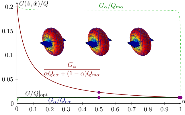
Fig. 20. G/Q determined from the dual problem (54) and bound (56) for a rectangular plate with side lengths \ell_x = 2\ell_y = \lambda/10 , direction \hat{r} = \hat{z} and polarization \hat{e} = \hat{x} (see Fig. 19). The maximal value is G/Q|_{\text{opt}} \approx 0.0123 giving Q \approx 125 and D \approx 1.53 .
