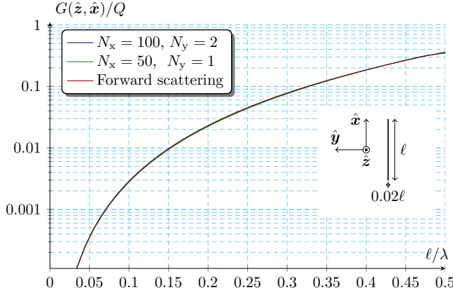
Fig. 16. Gain Q-factor quotient, G/Q , from the optimization problem (39) for a strip dipole with sides \ell \times \ell/50 , \ell/\lambda \leq 0.5 , \hat{\mathbf{r}} = \hat{\mathbf{z}} , \hat{\mathbf{e}} = \hat{\mathbf{x}} and N_x = \{50, 100\} . The forward scattering bound [32, 33] on G/Q is also included.
