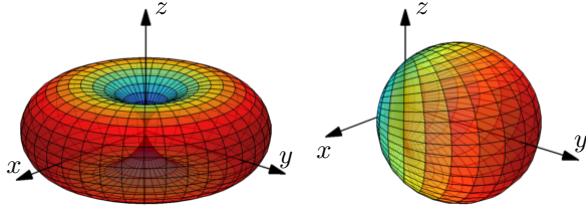
Fig. 24. Illustration of spherical modes. \hat{z} -directed electric dipole (left) and Huygens source composed of an \hat{x} -directed electric dipole and a \hat{z} -directed magnetic dipole (right).
