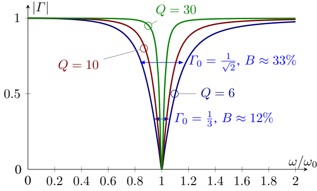
Fig. 7. Magnitude of the reflection coefficient |\Gamma| for RLC circuits with resonance frequency \omega_0 and Q-factors Q = \{6, 10, 30\} [37]. The fractional bandwidths (8) for the Q = 6 case with threshold levels \Gamma_0 = \{1/\sqrt{2}, 1/3\} are B \approx \{0.33, 0.12\} .
