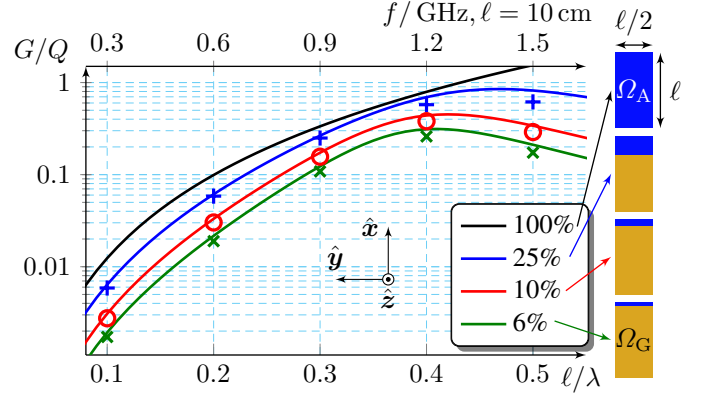
Fig. 6. Solid lines—physical bounds on G(\hat{z}, \hat{x})/Q for antenna regions \Omega_A restricted to rectangular regions. 6%, 10% and 25% of the region at the upper end in the l_x -direction is used for \Omega_A , cf. , Fig. 4. The situation with the entire region \Omega_A = \Omega used for optimization (100%) is included for comparison. Marks— G(\hat{z}, \hat{x})/Q values of structures optimized using a genetic algorithm (GA) [13, 14]. Insert—illustration of the considered situations. Blue and gold colored regions are the antenna \Omega_A and ground plane \Omega_G regions used in the convex and GA optimization (see also [37]).
