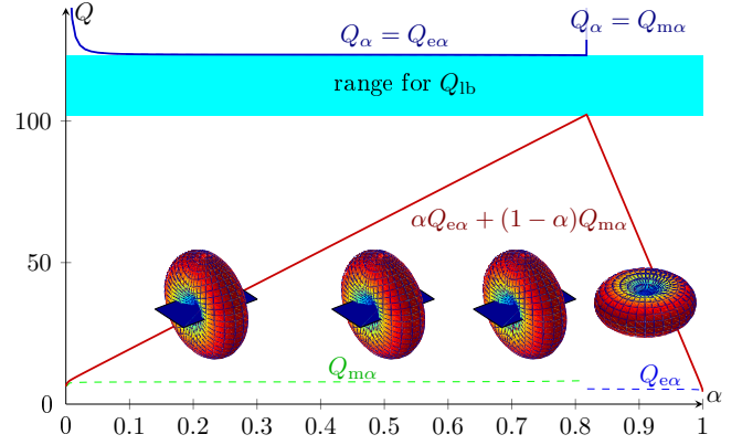
Fig. 25. Q-factor from the optimization problem (65) for the rectangular patch in Fig. 19. The parameters in (67) are depicted.
