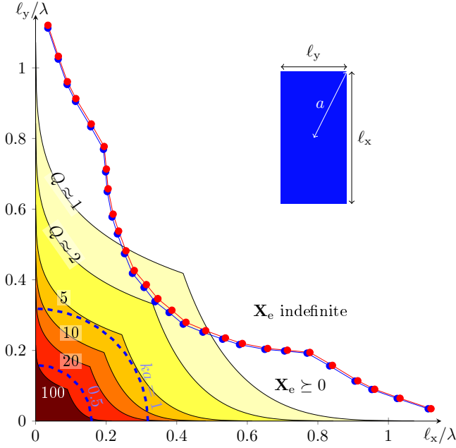
Fig. 30. Illustration of the maximal size of a planar rectangle with side lengths \ell_x and \ell_y such that \mathbf{X}_e is positive semidefinite \mathbf{X}_e \succeq 0 . The blue (red) curve with circular marks illustrate the largest (smallest) case with \mathbf{X}_e positive semidefinite (indefinite). The contours illustrate the region with Q \geq \{1, 2, 5, 10, 20, 100\} , where the Q-factor is estimated from the forward scattering bound [32, 33] assuming an electric dipole pattern. The classical regions for small antennas ka \leq \{0.5, 1\} are also depicted with the blue dashed quarter circles.
