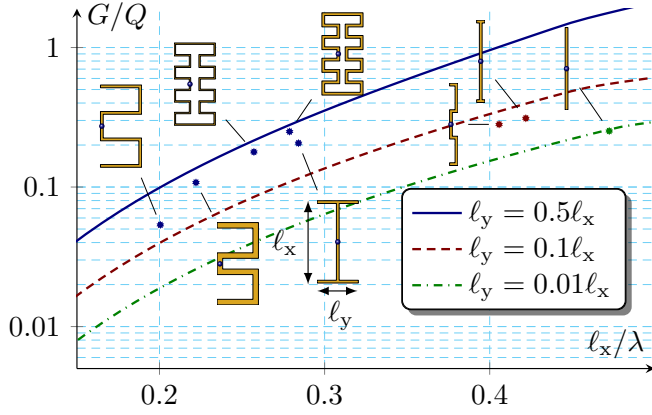
Fig. 5. Upper bounds on G(\hat{z}, \hat{x})/Q for rectangular plates with height l_x and widths l_y = \{0.5, 0.1, 0.01\}l_x , for l_x/\lambda \leq 0.5 , polarization \hat{e} = \hat{x} and radiation in the \hat{r} = \hat{z} direction. G/Q from simulations of PEC strip dipole, capacitive dipole, meander and folded meander antennas are included for comparison with the physical bounds. The antenna feeds are indicated with a dot. The size of the dipole is l_y = 0.01l_x , the other antenna dimensions are l_y = \{0.5, 0.1\}l_x with different line widths.
