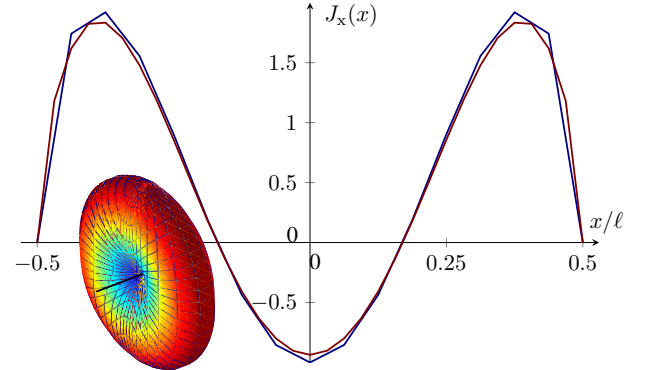
Fig. 12. Current distribution on the strip dipole with length \ell_x = \ell and width \ell/50 discretized with N_x = \{16, 32\} rectangles for the half wavelength case \ell/\lambda = 0.48 (wavenumber k\ell \approx 3 ). The radiation pattern, with D(\hat{z}, \hat{x}) \approx 2 , is also depicted.
