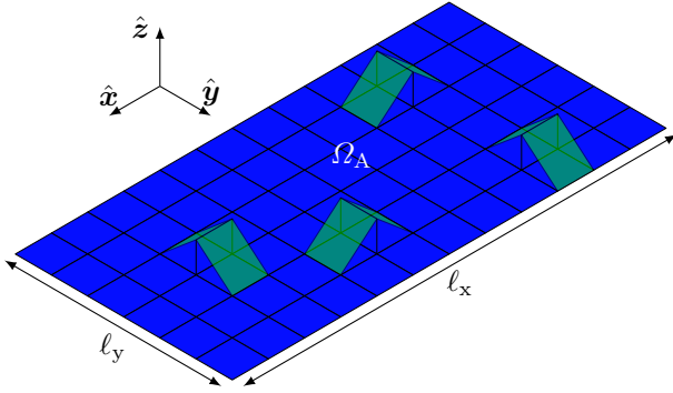
Fig. 17. A planar rectangular region with dimensions \ell_x \times \ell_y divided into N_x \times N_y = 12 \times 6 rectangular mesh elements. Four piecewise linear divergence conforming basis functions are depicted.
