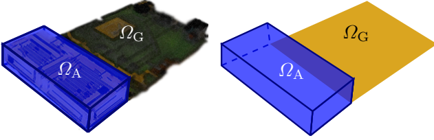
Fig. 4. Device geometry with a region \Omega with current density \mathbf{J} , (left) with a device and (right) the geometry. We assume that the currents \mathbf{J}_A can be controlled in the antenna region \Omega_A . The currents \mathbf{J}_G in \Omega_G = \Omega \setminus \Omega_A are induced by the currents \mathbf{J}_A (see also [37]).
